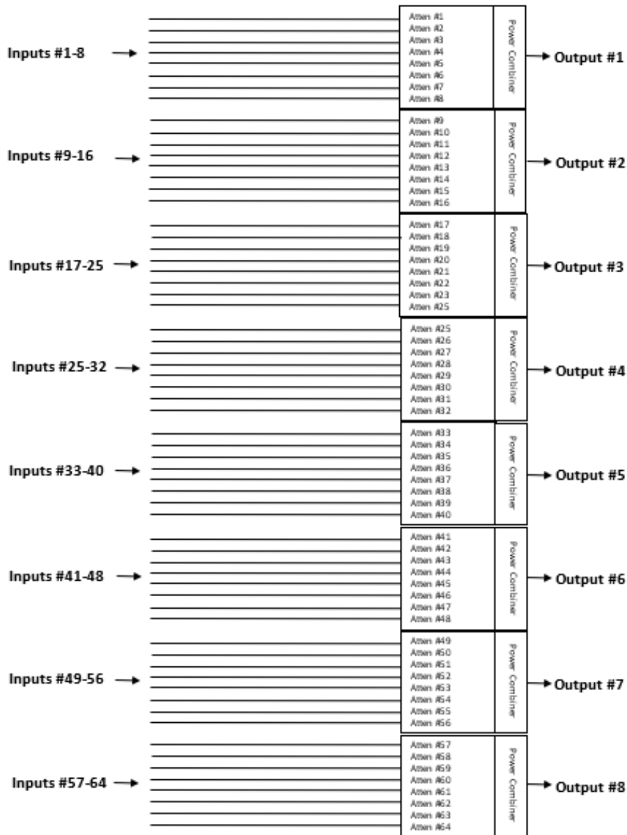
Functional Diagram
